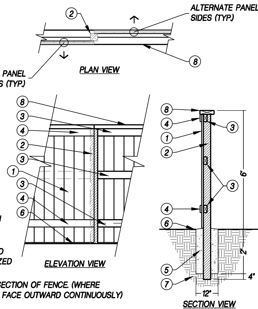
A ENHANCED WOOD FENCE WITH WOOD POST
